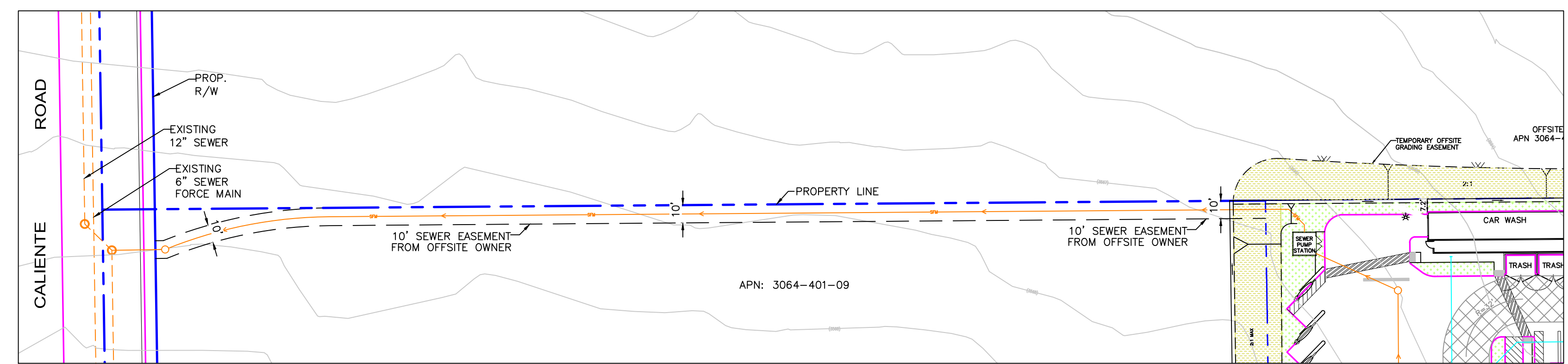
VIEW OF SEWER LATERAL WEST
