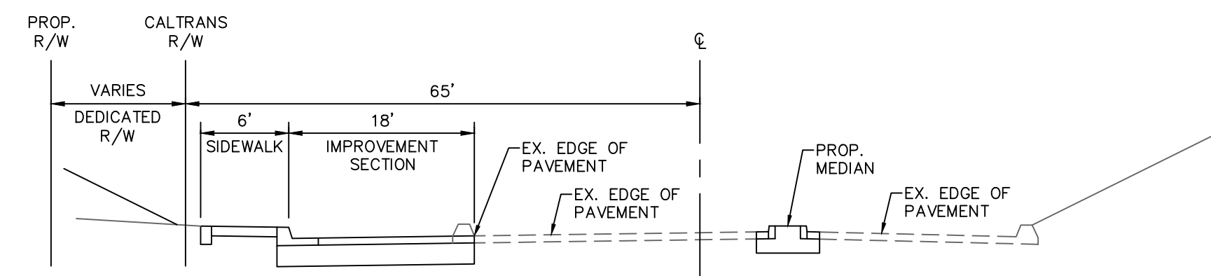
HIGHWAY 395 TYPICAL SECTION NOT TO SCALE
