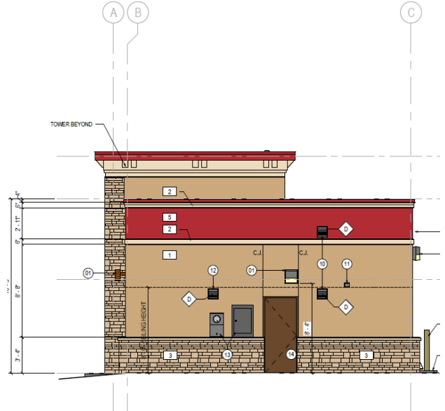
03 EAST ELEVATION SCALE: 1/4" = 1'-0"
