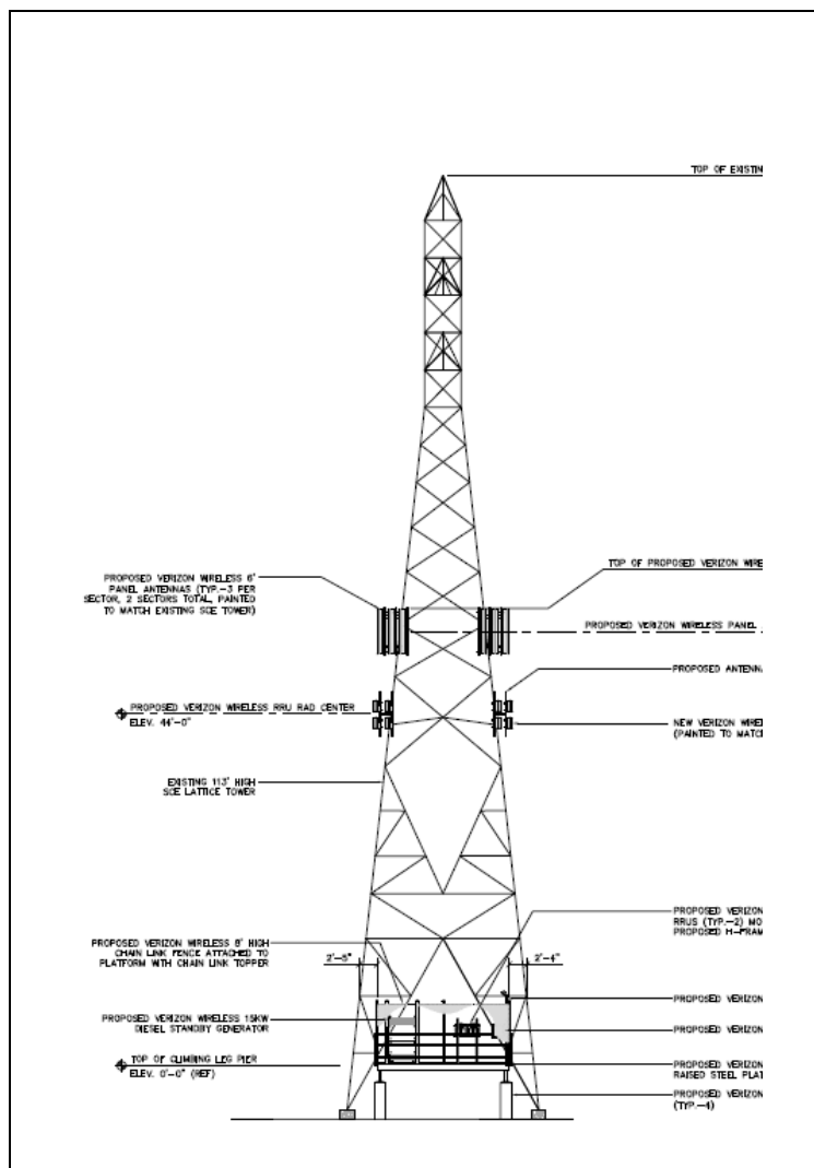
North Elevation
