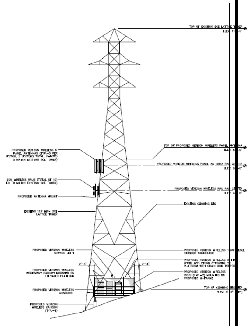
West Elevation
